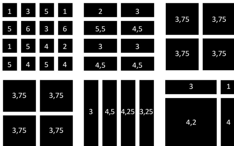
Figur 2. "The Modifiable Area Unit Problem" (MAUP).
